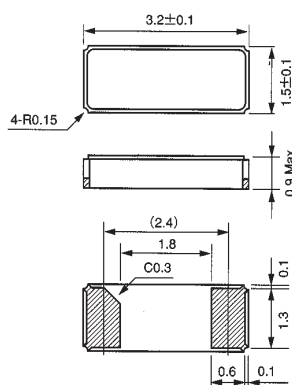
Dimensions (Units: mm)
