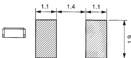
Recommended Solder Pattern
