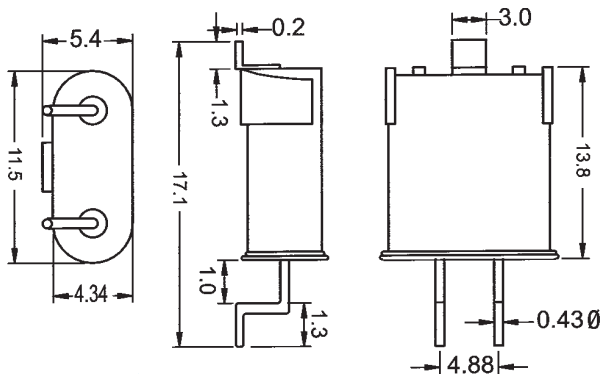
Package: HC-49/MJ
